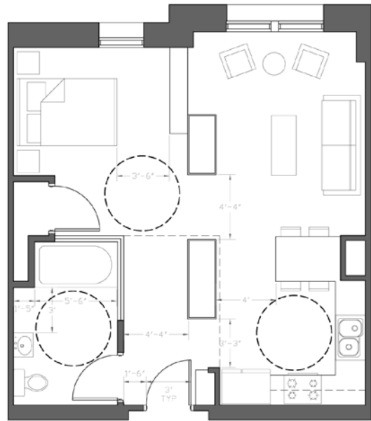
ACCESSIBILITY DIAGRAM 1/4" = 1'-0"
